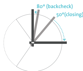
DAMPER CONTROL
