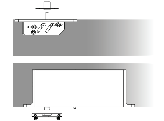
SYSTEM M STANDARD COMPONENTS : ceiling plate, top pivot, closer body, floor plate
